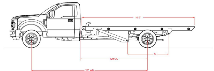
16 FT RAIL WITH FUEL TANK BEHIND CAB
