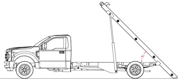
16 FT RAIL WITH FUEL TANK BEHIND CAB
