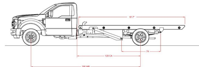
16 FT RAIL WITH FUEL TANK BEHIND CAB
